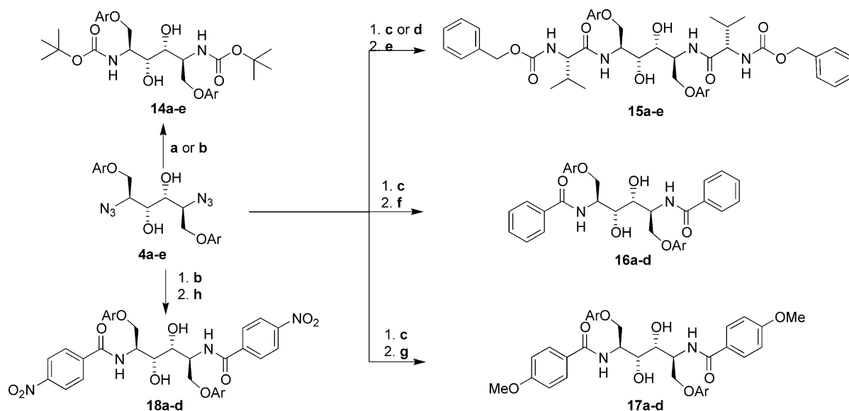
Scheme 3. Synthesis of compound set II, 14a–e , 15a–e , 16a–d , 17a–d and 18a–d (a) \text{H}_2 , Pd/C, (\text{Boc})_2\text{O} , EtOAc; (b) 1. \text{H}_2\text{S} , pyridine, \text{Et}_3\text{N} 2. (\text{Boc})_2\text{O} , \text{Et}_3\text{N} , EtOAc; (c) \text{H}_2 , Pd/C, EtOAc; (d) \text{H}_2\text{S} , pyridine, \text{Et}_3\text{N} ; (e) Z-Val-OH, PyBOP, DIPEA, \text{CH}_2\text{Cl}_2 ; (f) benzoic anhydride, \text{CH}_2\text{Cl}_2 ; (g) 4-methoxybenzoic anhydride, \text{CH}_2\text{Cl}_2 ; (h) 4-nitrobenzoic anhydride \text{CH}_2\text{Cl}_2 .
