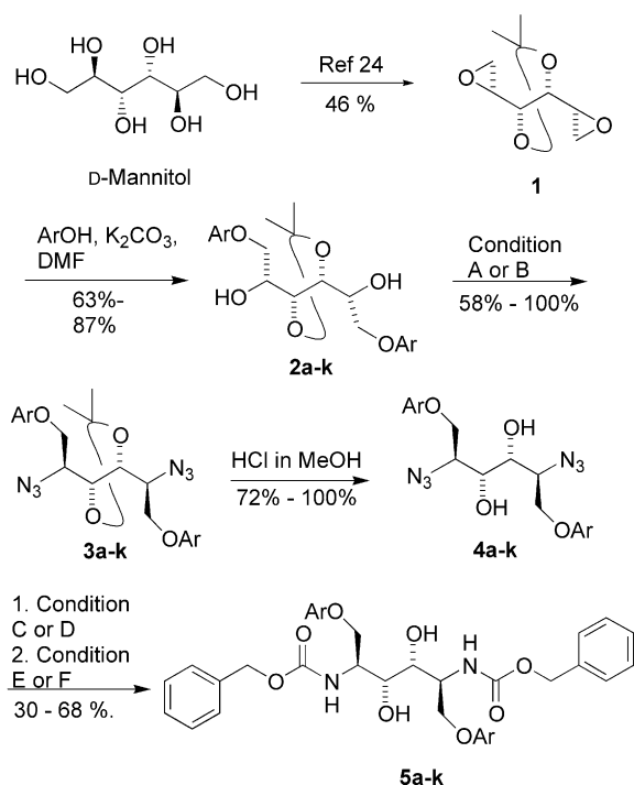
Scheme 1. Synthesis of compound set I, 5a–k . Condition: (A) Ph 3 P, DIAD, THF; (B) 1. Tf 2 O, pyridine, CH 2 Cl 2 2. NaN 3 , DMF; (C) 1. H 2 , Pd/C, EtOAc 2. benzyl chloroformate, pyridine, CH 2 Cl 2 ; (D) 1. H 2 S, pyridine, Et 3 N 2. N -(benzyloxycarbonyloxy)-succinimide, Et 3 N, CH 2 Cl 2 .
