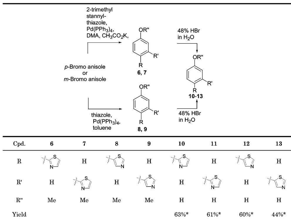
Scheme 2. Synthesis of phenols 10–13 ; * overall yields.
